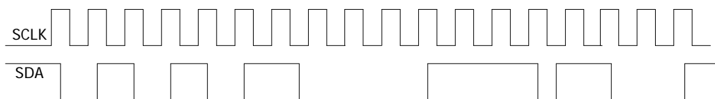
Figure 12-5 I2C Serial Bus
