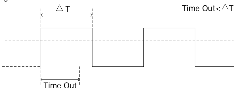
Figure 5-8 Timeout Trigger
